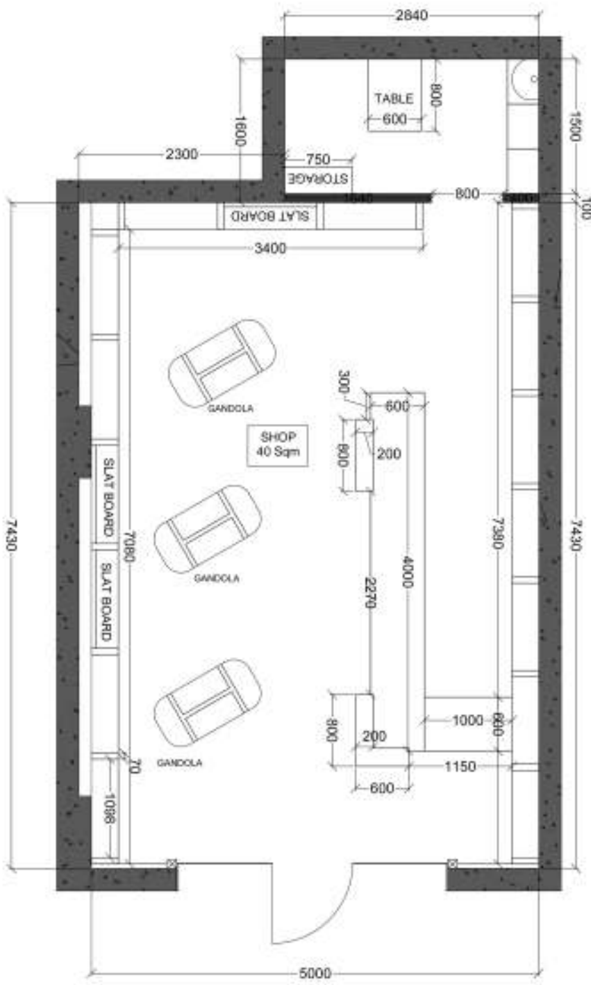
PLAN
