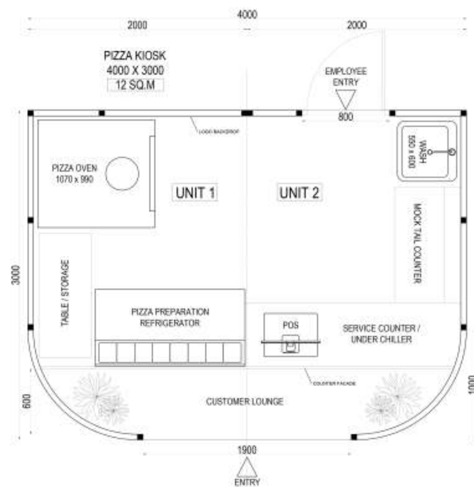
PLAN
