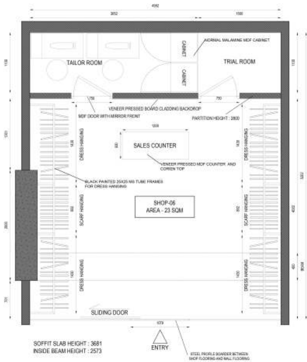
PLAN
