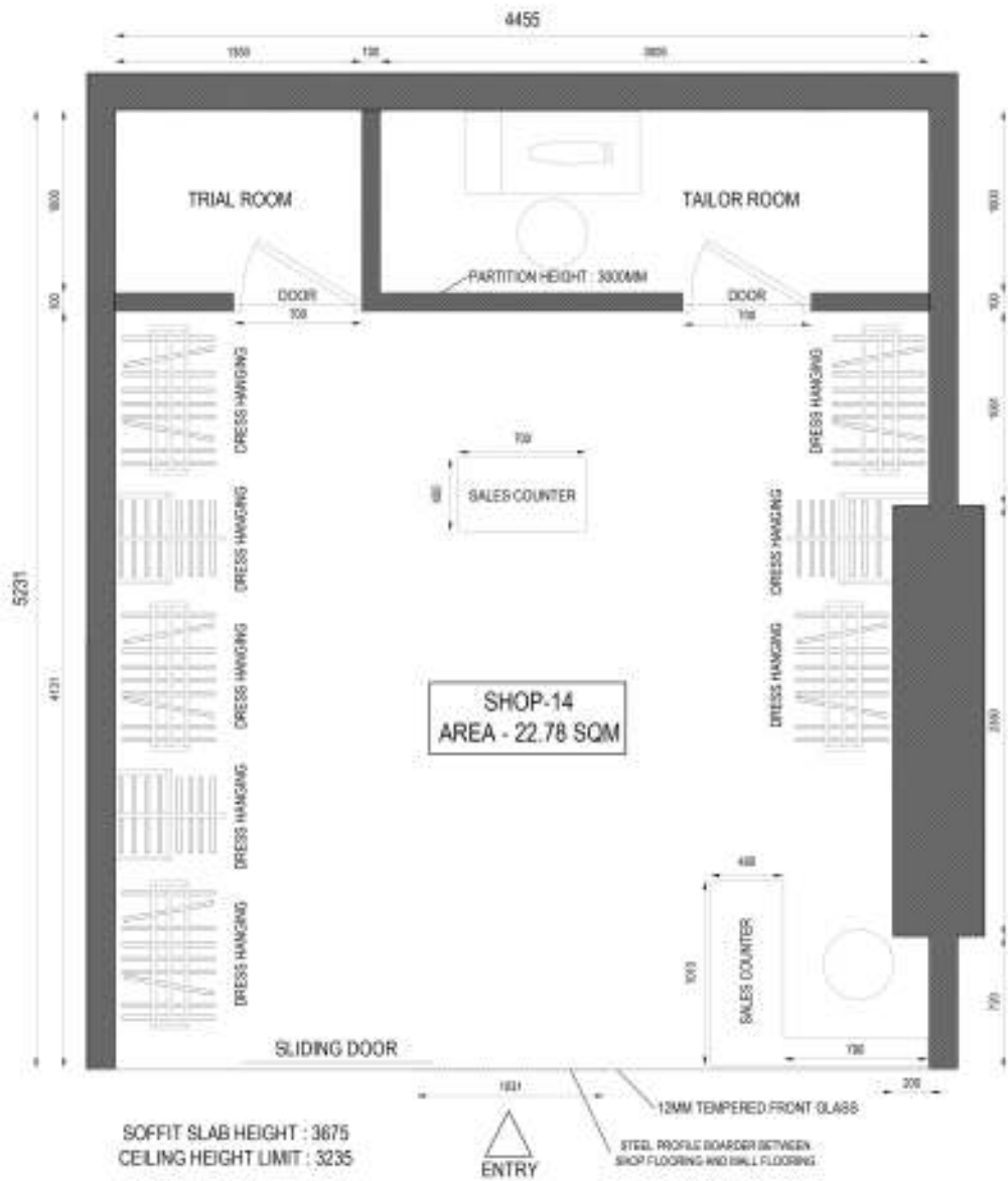
PLAN
