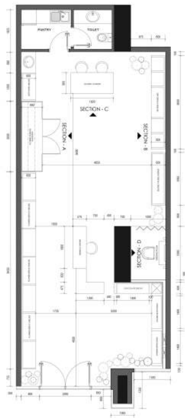
PLAN
