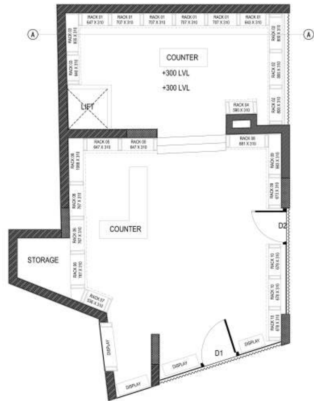
PLAN
